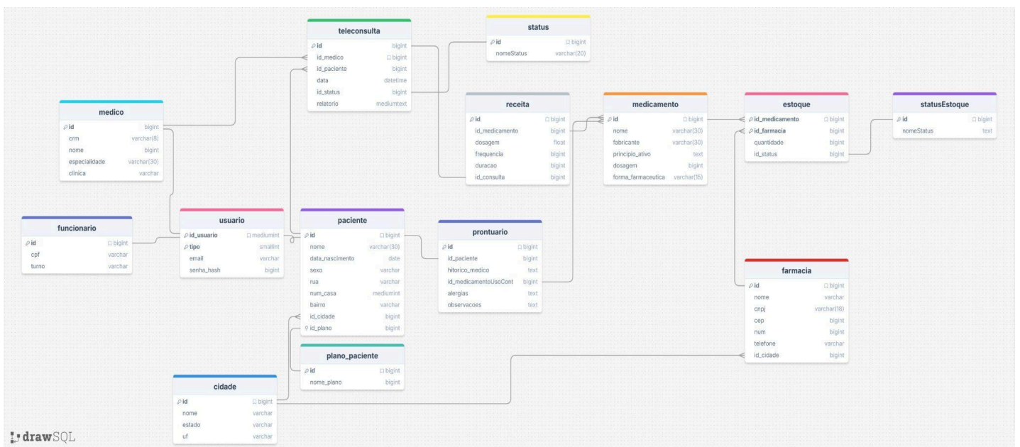
Figura 22 - MER FarmaGrid+
